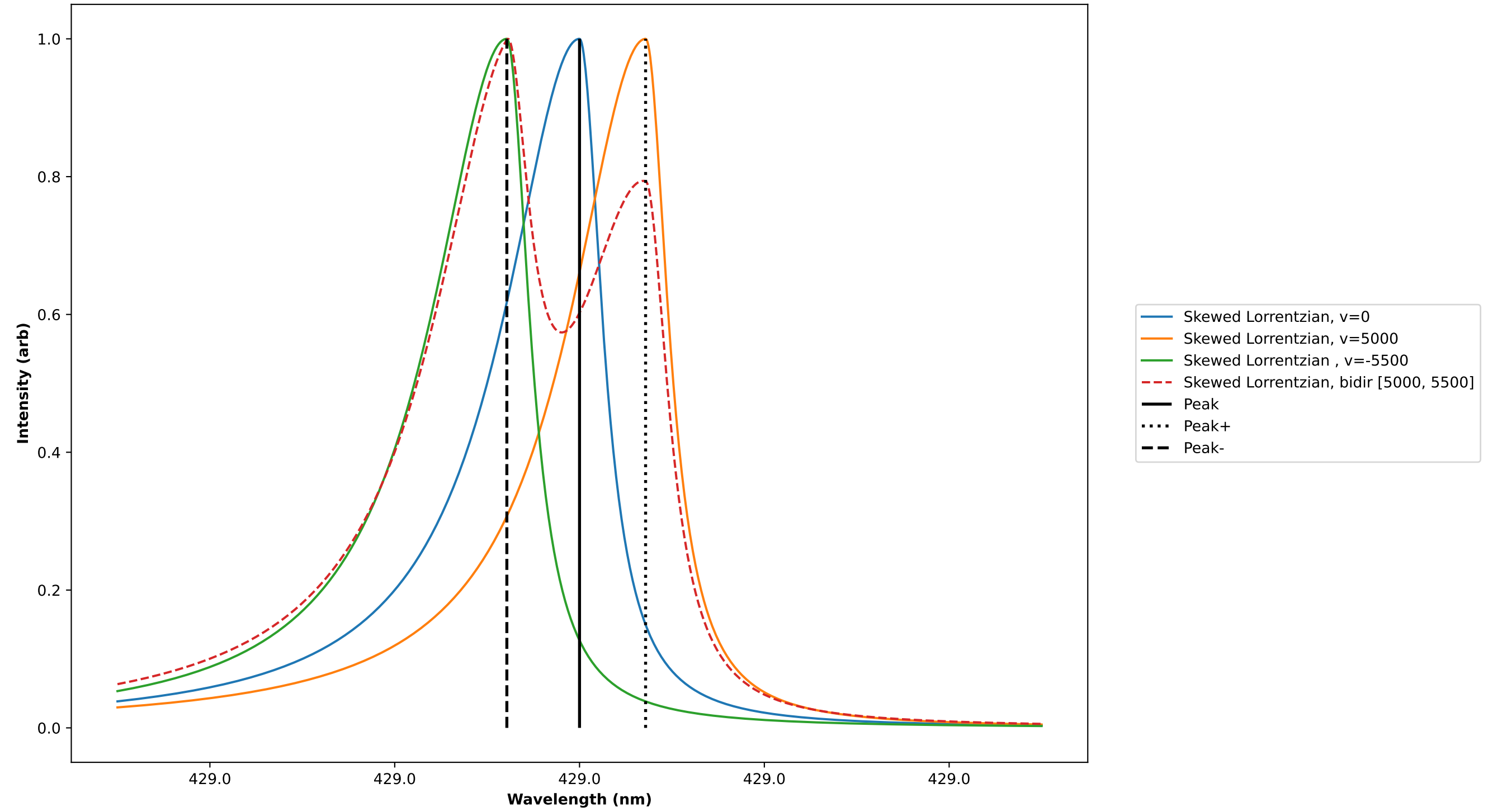
Skewed Lorentzian: T=10.0 eV, AMU = 183, Pixels = 0.01 nm, Skewness = [1, 0.3]
